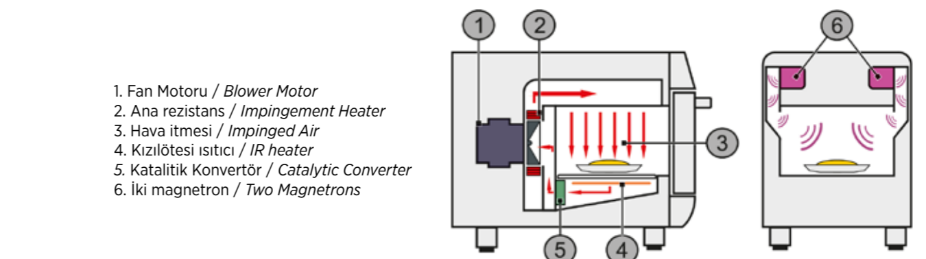
Chef Express Teknik İllüstrasyonu Technical Illustration of Chef Express
